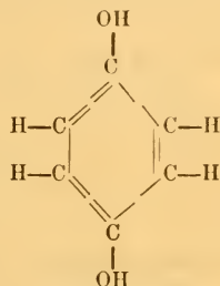
Hydroquinone.
